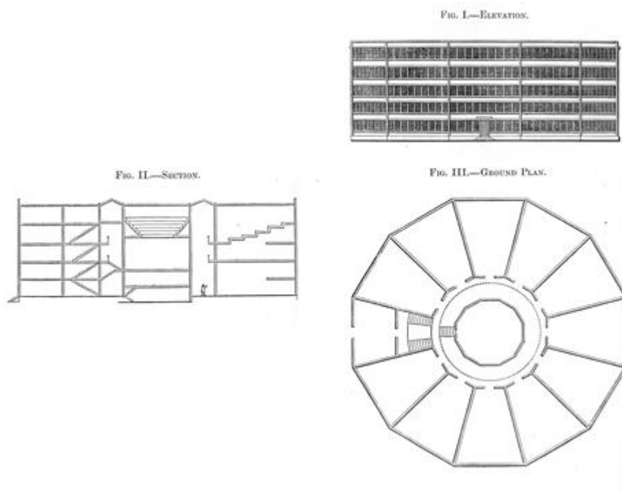
Figure 5: Samuel Bentham with Samuel Bunce, project for a House of Industry, 1797: plan, section and elevation. 25
