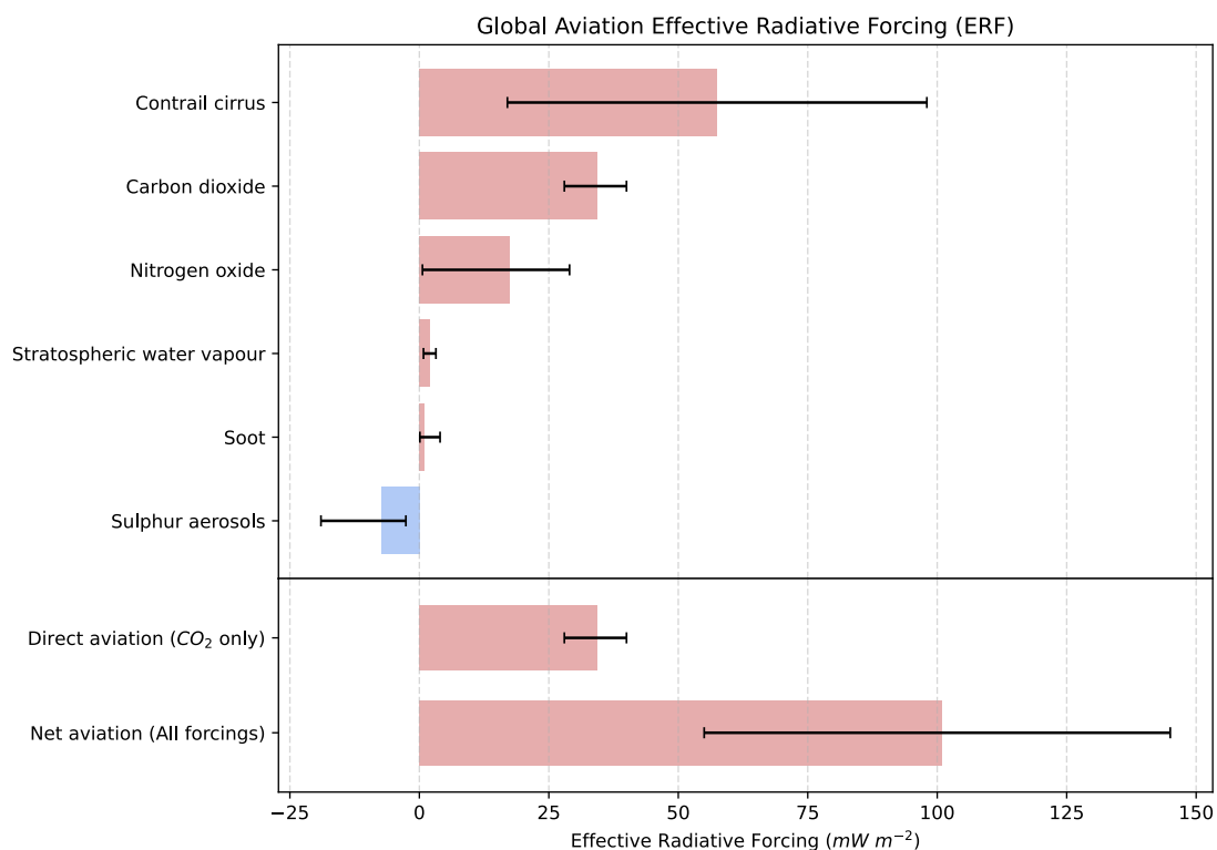
460 Figure 5: Best estimates of effective radiative forcing (ERF) of aviation between 1940-2018 (Adapted from ref 25). Red bars indicate a warming effect, blue bars indicate a cooling effect. Whiskers indicate the 5-95% confidence interval.
