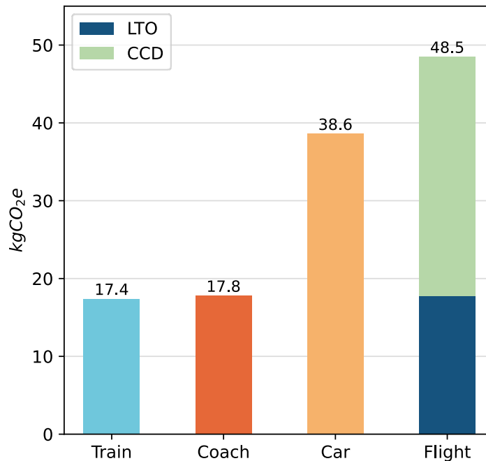
Figure 3: The carbon footprints associated with various modes of transport between London and Glasgow. Includes emissions associated with the landing-take-off (LTO) and climb-cruise-descent (CCD) phases of flight.
