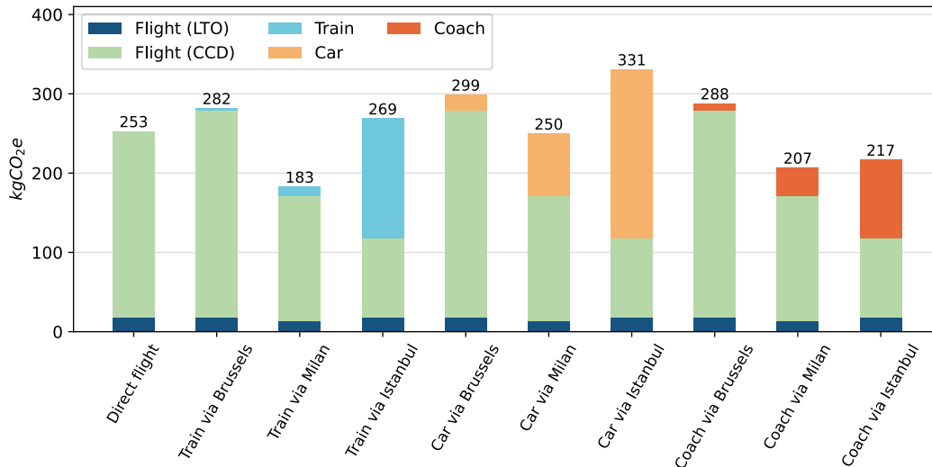
360 Figure 2: A selection of journeys between London and Sharm El-Sheikh and their associated carbon footprints, coloured by mode of transport. Includes emissions associated with the landing-take-off (LTO) and climb-cruise-descent (CCD) phases of flight. Routes ‘via’ a waypoint travel by the specified land transport up to the waypoint before flying the remainder of the route to Sharm El- Sheikh. All flights are economy seats, and all car journeys are calculated for a diesel Ford Fiesta with two passengers.
