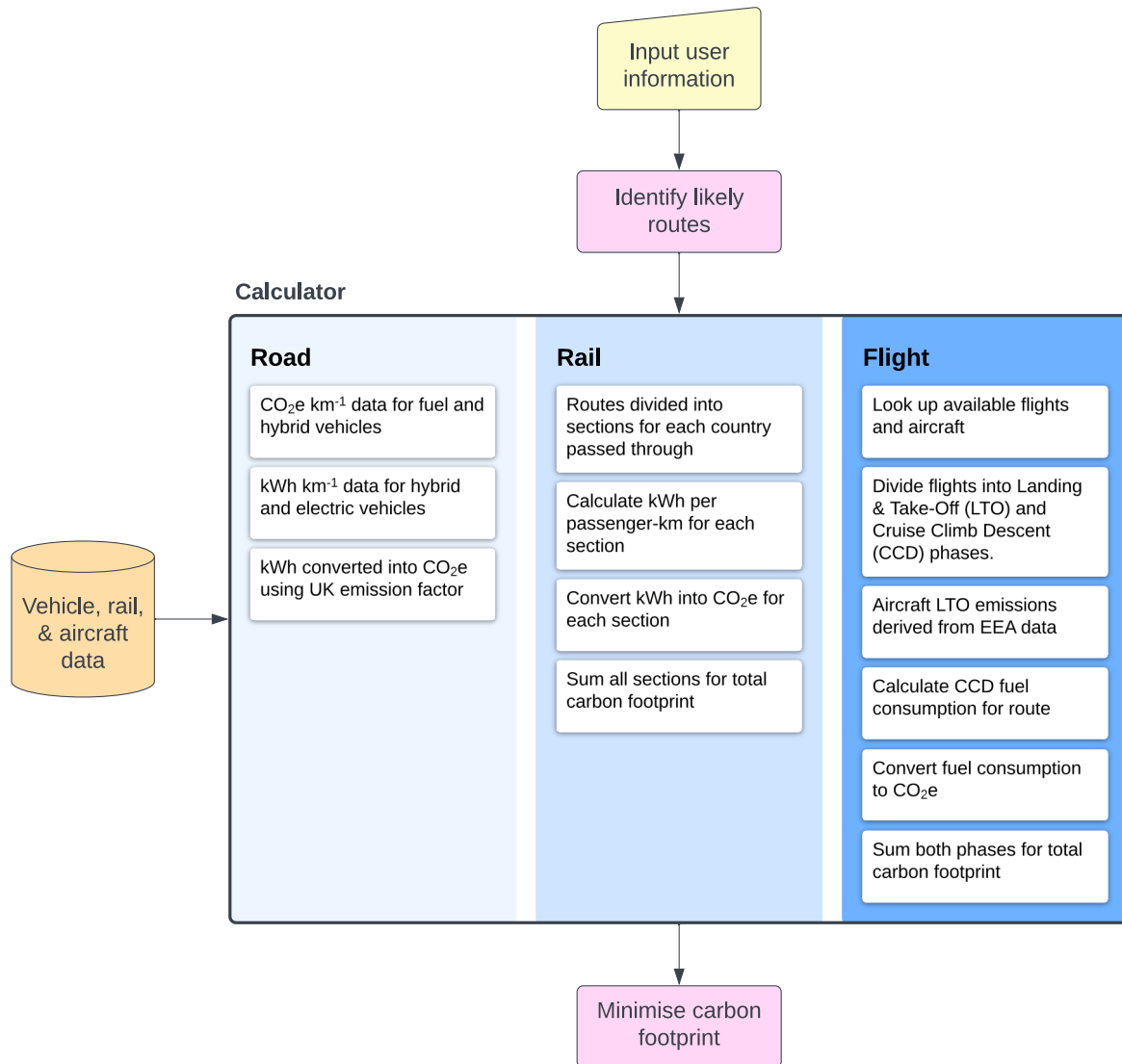
175 Figure 1: Flow chart representing the carbon footprint calculator, flowing from top to bottom. Model components are represented in shades of blue (coach and passenger car both represented by 'Road'), with important features listed.
