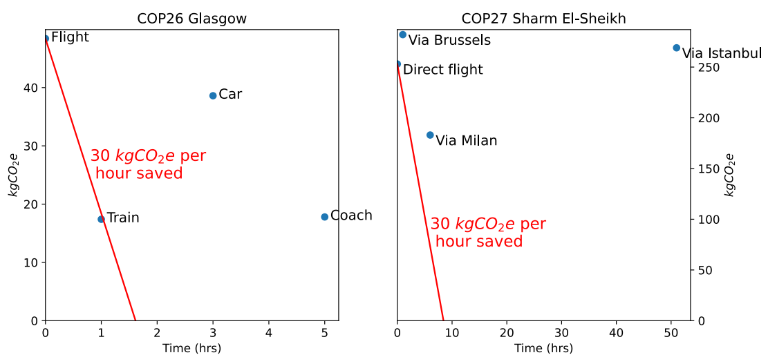
405 Figure 4: The carbon footprint of various routes to (left) Glasgow and (right) Sharm El-Sheikh from London, plotted against the length of the journey in hours. The red line indicates points equal to a 30kgCO 2 e per hour saving from the direct flight option in each case. The COP 27 routes utilise rail transport up to the specified city, then fly direct to Sharm El-Sheikh.
